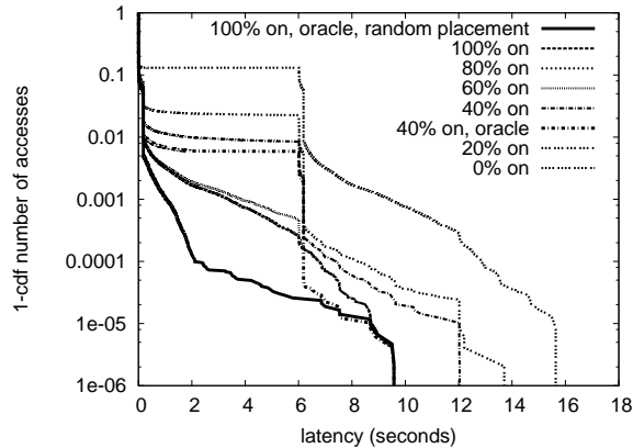
Figure 2: CCDF: Effect of increasing percentage of powered-up disks on performance.
