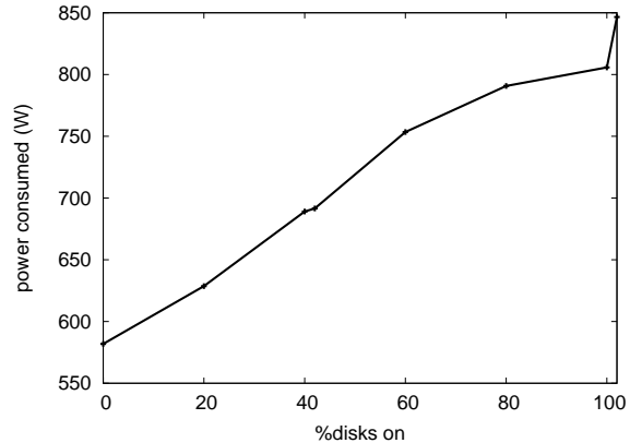
Figure 3: Effect of increasing percentage of powered-up disks on power consumption
